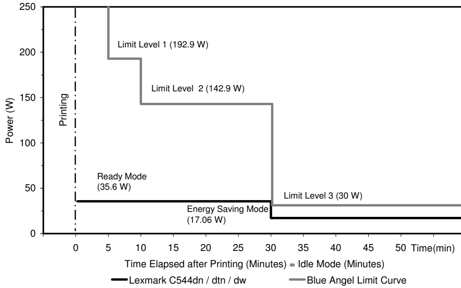
Power Consumption and Default Times of the Lexmark C544dn / dtn / dw during time elapsed after last print
