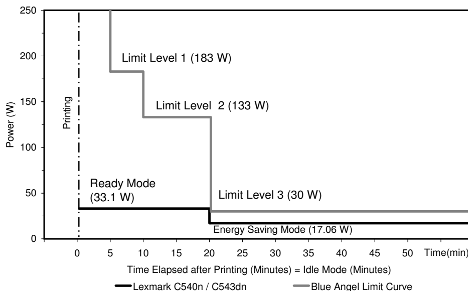
Power Consumption and Default Times of the Lexmark C540n / C543dn during time elapsed after last print
